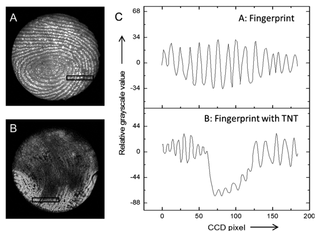
Figure 7. Detection of residues of TNT ( 10 \mu\text{g mL}^{-1} in methanol) on a fingerprint by using the ECL-based image-contrast technique. A) Positive ECL image of a LFP on pSi. B) ECL image of the LFP on pSi impressed with the same fingertip pretreated with TNT. C) Cross-sectional relative gray values over 15 parallel ridges within the area indicated by the black rectangles in (A) and (B). ECL measurements were performed in 1 M \text{KNO}_3 with an applied potential of 0.8 V.
